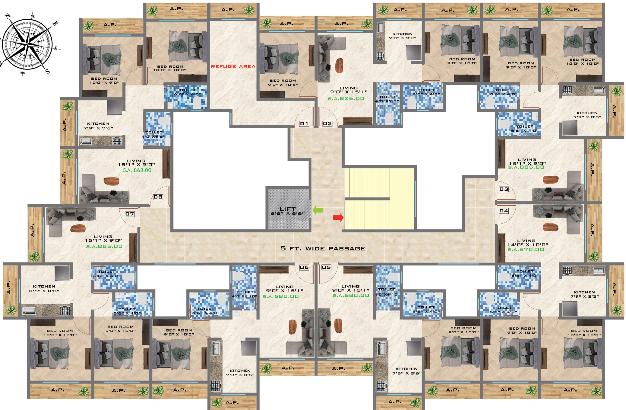
TYPICAL FLOOR PLAN FLOOR PLAN FOR 7TH FLOOR
